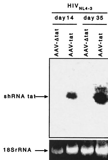
FIG. 4. Northern blot analysis of tat shRNA expression in HIV-1 NL4.3 -infected H9 cells transduced with AAV- tat or AAV- \Delta tat . Continuous expression of tat shRNA was observed on days 14 and 35 after HIV-1 NL4.3 infection. rRNA expression was used as a loading control.
