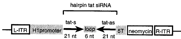
FIG. 1. Schematic representation of a short hairpin siRNA expression cassette introduced within the ITRs of a recombinant AAV-2 DNA vector. The H1 promoter was used to express tat siRNA in the form of a hairpin transcript consisting of a 21-nucleotide (nt) sense and 21-nucleotide antisense sequence separated by a hexaloop (5'-CTG CTT GTA CCA ATT GCT ATT AGG ATC AAT AGC AAT TGG TAC AAG CAG TTT TT-3'). A five-thymidine transcription termination signal was placed downstream of the hairpin sequence. To allow the generation of shRNA-expressing cell lines, an SV40 early promoter-driven neomycin resistance gene was introduced downstream of the hairpin expression cassette.
