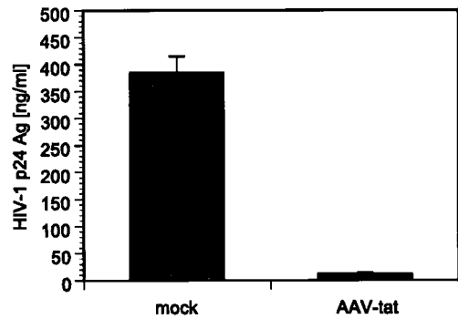
FIG. 3. To verify the antiviral activity of H1 promoter-driven tat siRNA, 293T cells were cotransfected with HIV-1 NL4.3 and pAAV DNA constructs. Quantification of viral p24 antigen levels 48 h posttransfection in cell-free supernatant revealed a 97% decrease in cells expressing tat shRNA (pAAV- tat ) compared to cells that were transfected with HIV-1 NL4.3 and control mock vector lacking tat -specific sequences (pAAV- \Delta tat ). Values represent averages of three independent experiments, with the ranges indicated.
