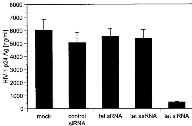
FIG. 2. Cotransfection of various synthetic RNA species including tat -specific sense (s), antisense (as), and short interfering (si) molecules with HIV-1 NL4.3 in 293T cells. An siRNA with no sequence homology to HIV-1 was included as a control. Cell-free supernatant was assayed for HIV-1 p24 antigen (Ag) levels on day 4 posttransfection and demonstrated 91% reduction of p24 in cells transfected with tat siRNA compared to controls. Values represent averages of three independent experiments, with the ranges indicated.
